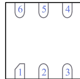
SJT5233DS DFN6L (Top View)
